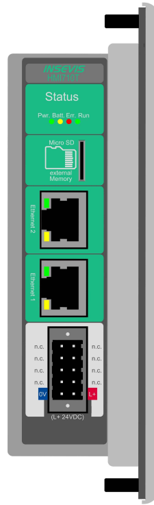
Figure above: View to rear side and connections sides of HMI710T (horizontal use)
